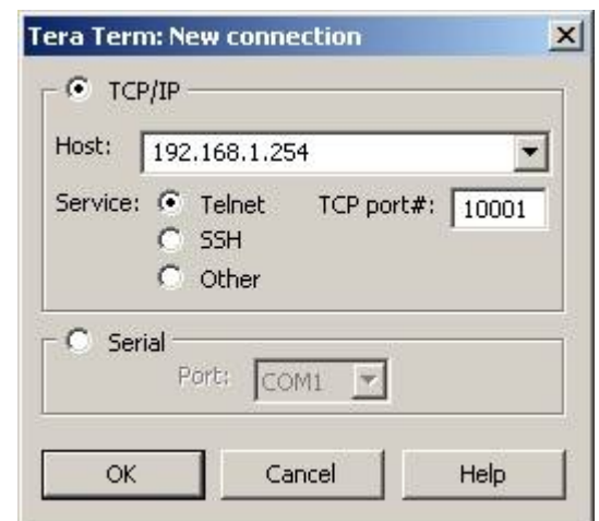
Fig. 36 – New connection
