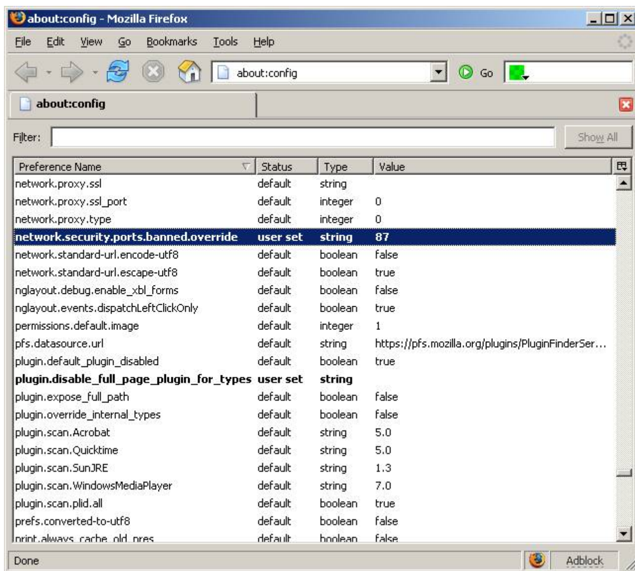
Fig. 8 – Example of Firefox browser with port 87 enabled
