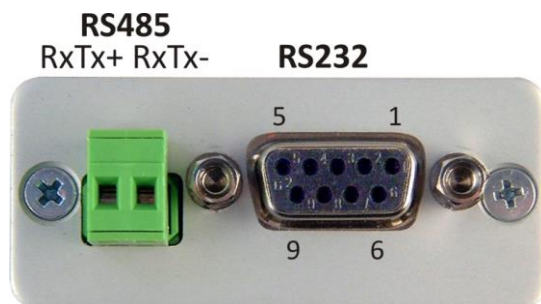
Fig. 7 – Terminals for RS232 and RS485 2 serial lines connection
