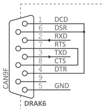
Fig. 8 – RS232 connector diagram
